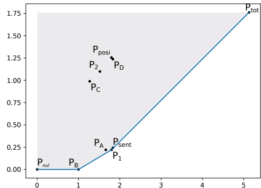
Figure 1: I_L(P) - I_{\bar{L}}(P) represented w.r.t. I_L(P) for different partitions: acceptable solutions of program (1) lie on the convex hull boundary of the set of all partitions. Solution for \gamma is given by the tangent of slope \gamma . Non trivial solutions are P_B and P_1 .
